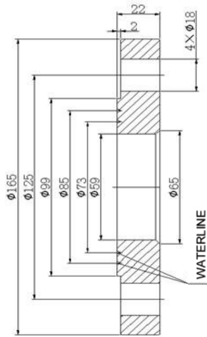
Figure 1, Density Meter Dimension
