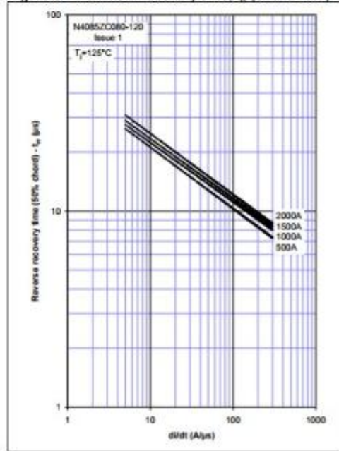
Figure 8 - Maximum recovery time, t_{rr} (50% chord)
