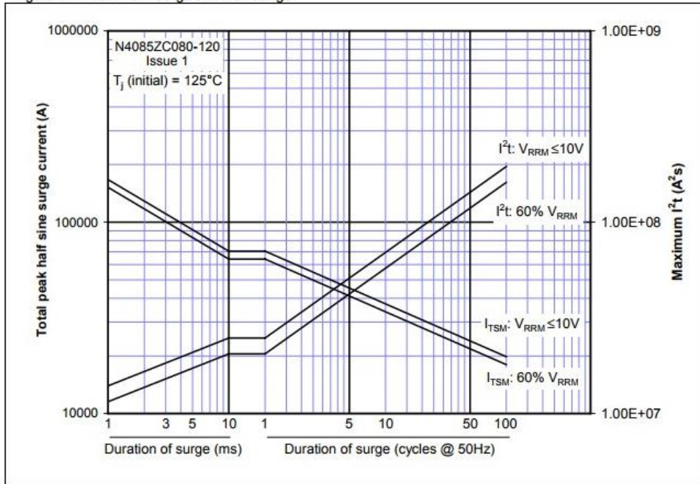
Figure 17 - Maximum surge and I^2t Ratings
